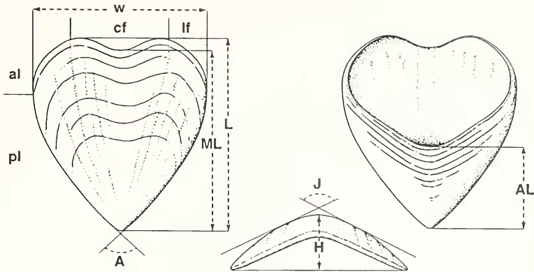
TEXT-FIG. 2. Schematic diagram of intermediate sclerite of Chelodes showing standard measurements and terminology in dorsal (left), ventral (right) and posterior (middle) views. L = length; ML = median length; W = width; AL = apical length; H = height; A = apical angle; J = jugal angle; al = anterolateral and pl = posterolateral portions of lateral margins; cf = central shell field; lf = lateral shell field.
